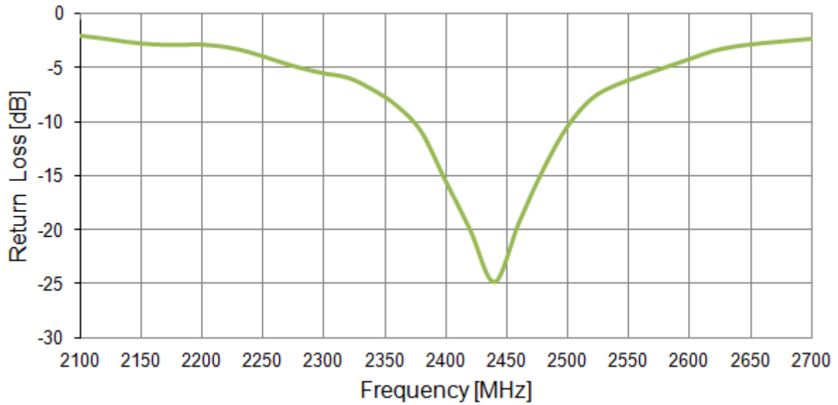
Figure 2. Return loss of the FXP840 antenna from 2100 MHz to 2700 MHz.
