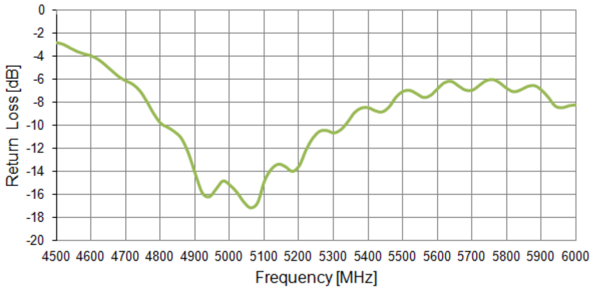
Figure 3. Return loss of the FXP840 antenna from 4500 MHz to 6000 MHz.
