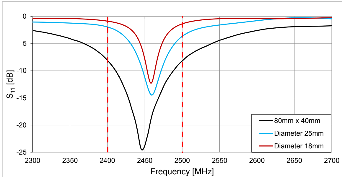
Figure 26. S_{11} Plot for 2400-2500MHz band
