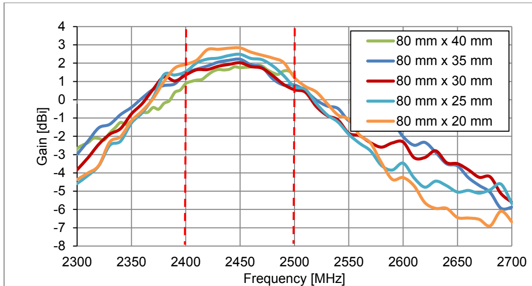
Figure 17. Peak Gain plot for 2400-2500MHz band
