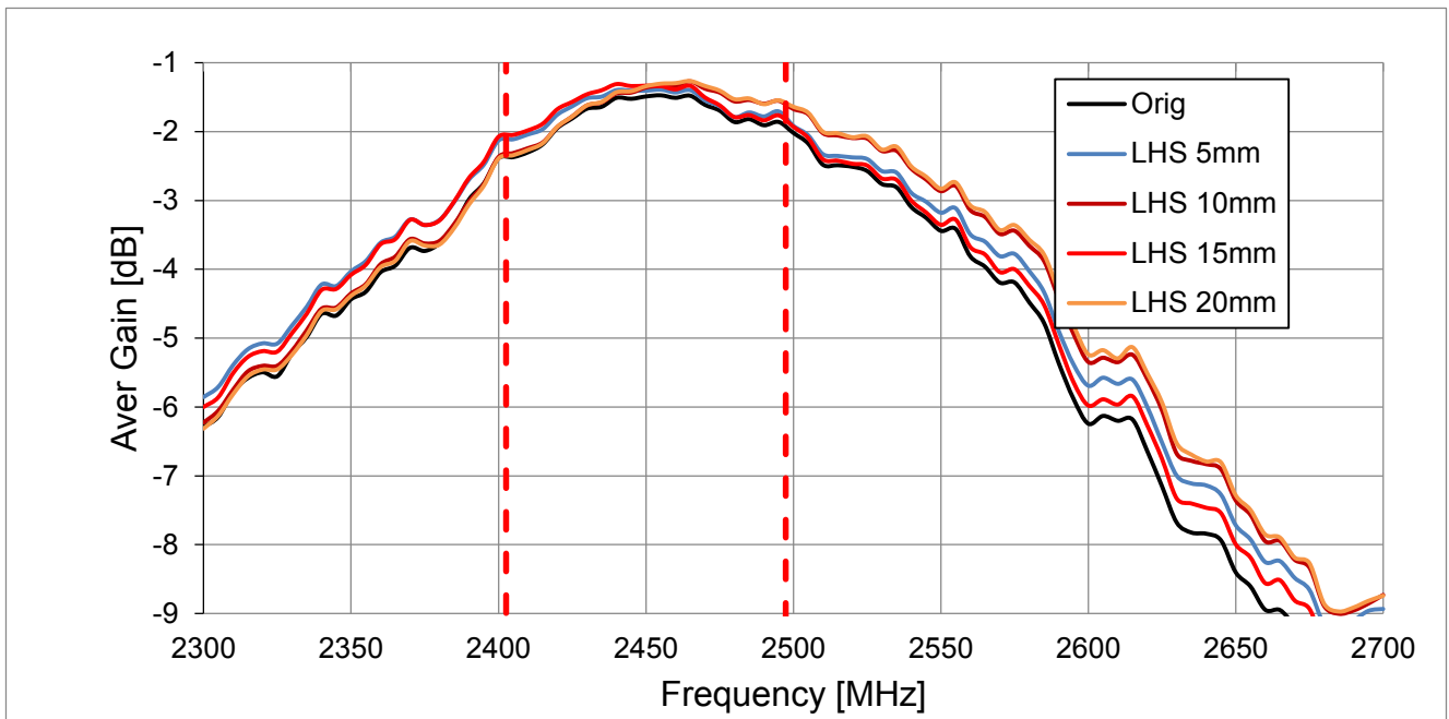
Figure 46. Average Gain plot for 2400-2500MHz band
