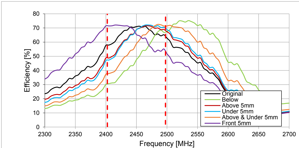
Figure 49. Efficiency plot for 2400-2500MHz band
