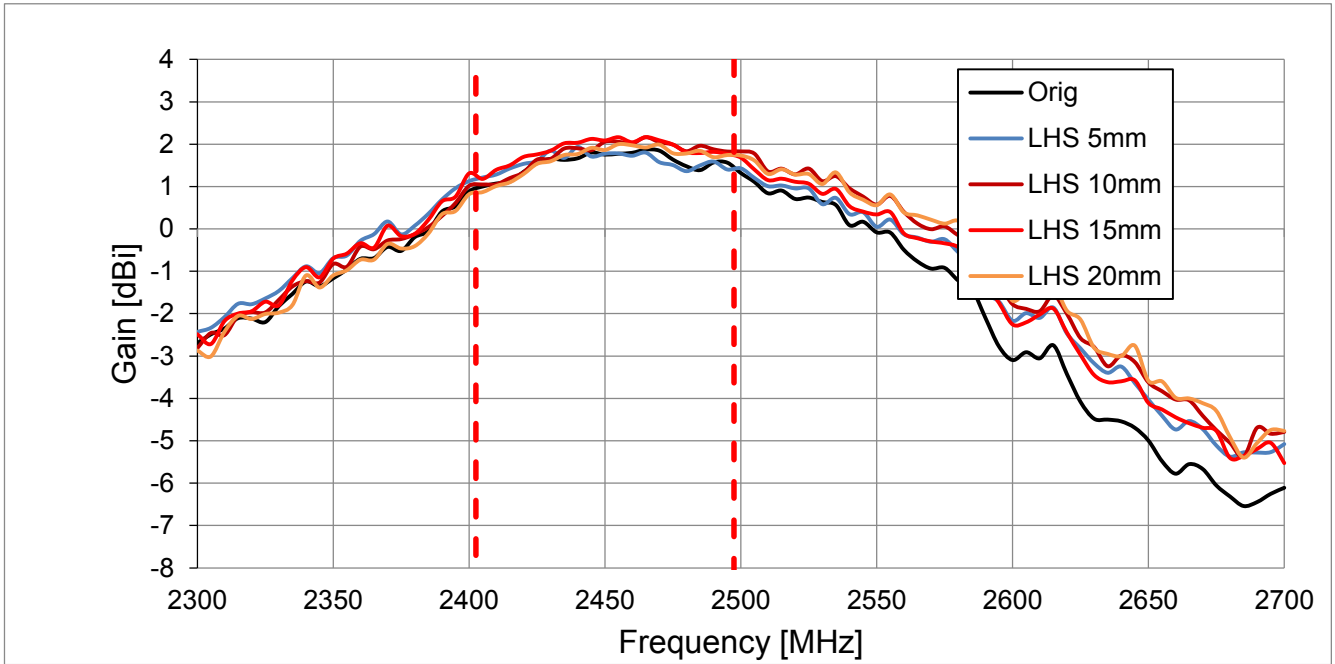
Figure 45. Peak Gain plot for 2400-2500MHz band
