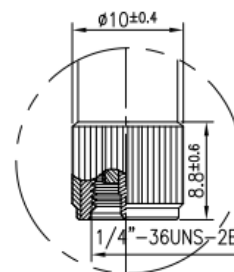
SMA(M) Connector (New)
