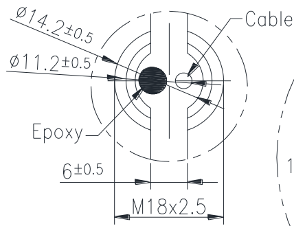
Bottom Thread View
