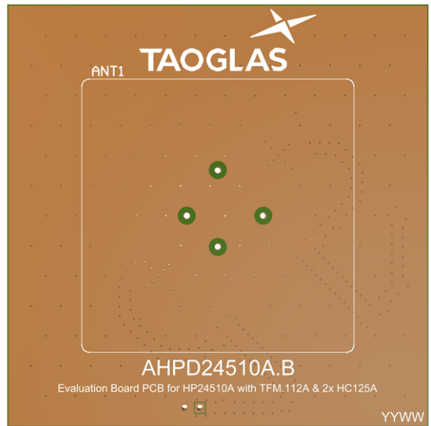
Top Side ( HP24510A placement on 70x70mm PCB)
