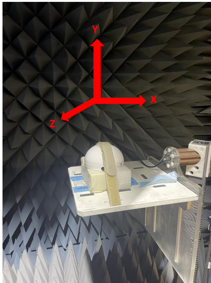
Chamber Test-Setup
