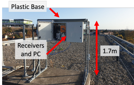
Fig. 2. GNSS receiver setup, Taoglas Office Dublin, Ireland.
