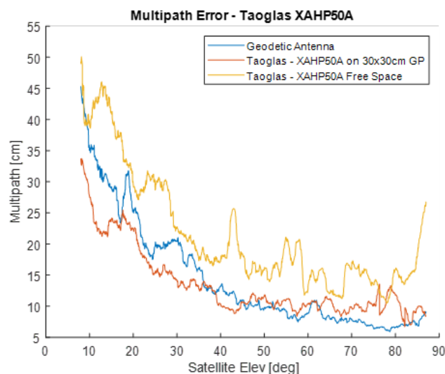
Fig. 7. Standard deviation of the multipath error for GPS L1-C/A signal. Ground plane effect on Taoglas XAHP.50A.
